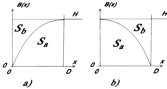
FIG. 6. (a) The flux profiles when the field H=H^* is applied after cooling in zero field [or when temperature in ZFC measurements reaches the value T^* , defined by H^*(T^*)=H ]. (b) The flux profile after cooling in field H , and removing this field at temperature T^* . In case (a) M_{ZFC} is proportional to the surface S_b , while in case (b) M_{rem} is proportional to the surface S_a .
