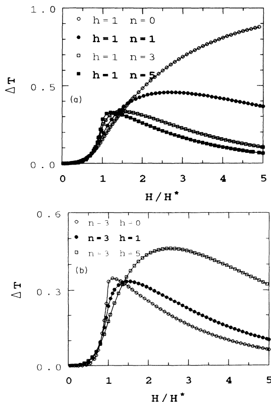
FIG. 9. The temperature change \Delta T (in normalized units) as a function of field, when the relaxation time is given by 1/\tau=0.5 . (a) h=1 and n changes between 0 and 5, (b) n=3 but h changes from 0 to 5.
